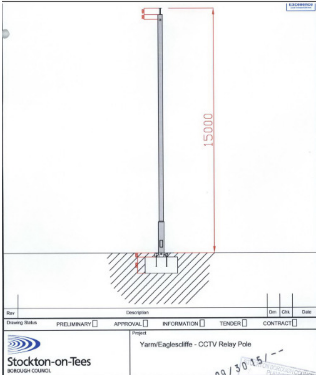
Drawing No 1; Relay Pole Detail
